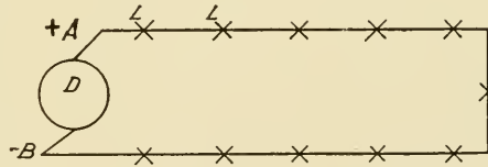
Fig. 3. Diagram of Series Distributing System
